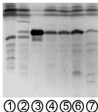
Figure 4.2 High performance TLC of fractionated commercial \beta -GluCer. Each numbered lane (10 \mu g of material per lane) roughly represents the following eluents (in ascending order) 5% MeOH/DCM, 10% MeOH/DCM, 20% MeOH/DCM, 40% MeOH/DCM, 25:65:2 MeOH:DCM:H 2 O, 25:65:4 MeOH:DCM:H 2 O, and 65:25:10 MeOH:DCM:H 2 O
