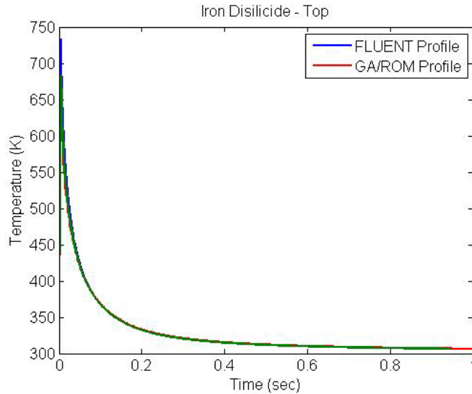
Figure 4-2: Iron Disilicide Top Temperature Profile Comparisons
