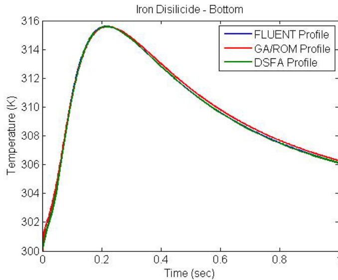
Figure 4-1: Iron Disilicide Bottom Temperature Profile Comparisons
