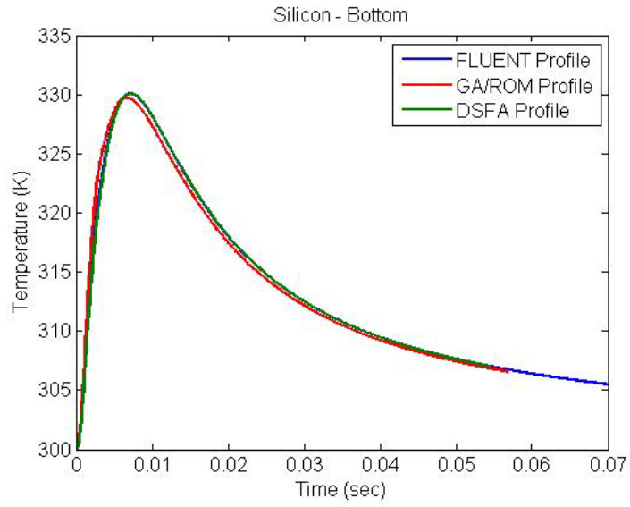
Figure 3-24: Silicon Bottom Temperature Profile Comparisons
