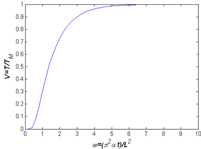
Figure 2-2: Nondimensional Temperature Rise from Parker Equations
