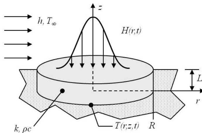
Figure 3-6: DSFA Model of PLD Schematic
