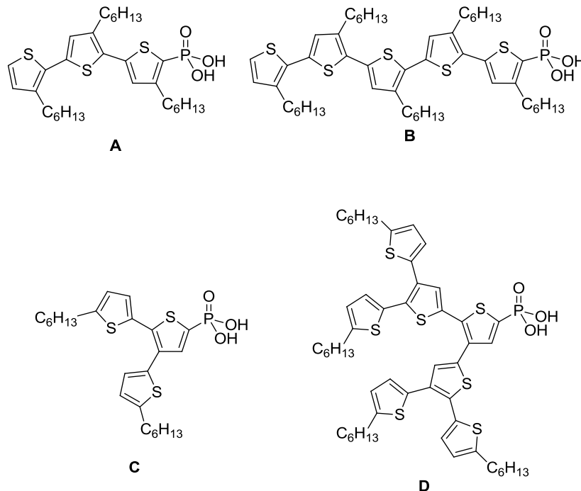
Figure 1.10. Oligothiophenes used by Milliron 21 (A,B) and Locklin 22 (C,D) in solar cells using a phosphonic acid anchor.
