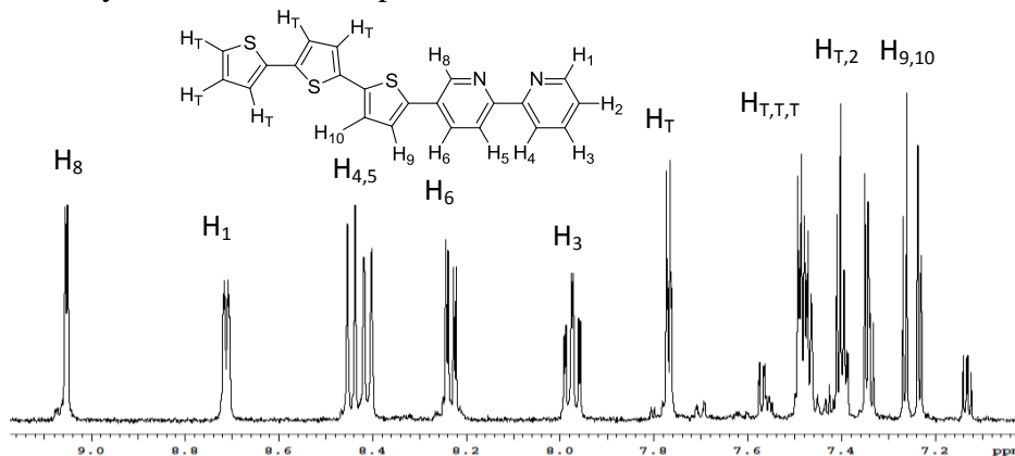
Figure 1.21. ^1\text{H} NMR of 5-T 3 bpy.
