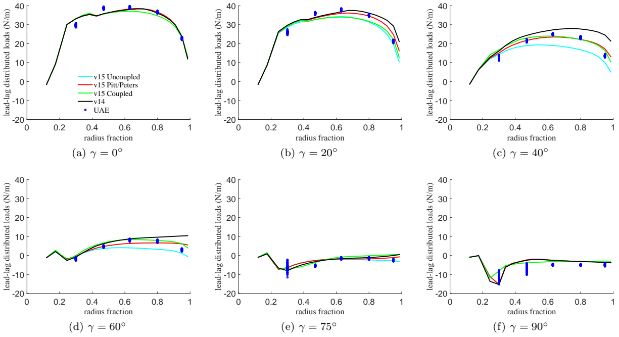
Figure 10: Distributed lead-lag loads along blade at six different yaw angles ( V_\infty = 7 m/s, \psi = 270^\circ ).
