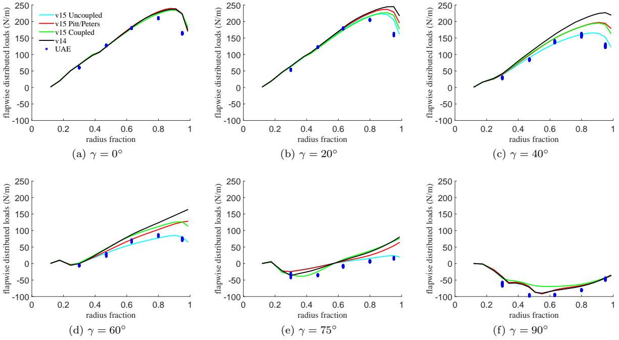
Figure 11: Distributed flapwise loads along blade at six different yaw angles ( V_\infty = 7 m/s, \psi = 270^\circ ).
