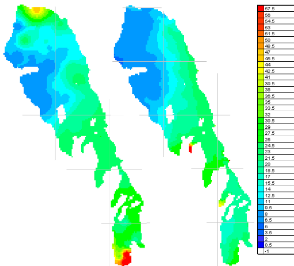
Figure 10. Lake Winnipeg TSS October 2002 Observed and PolTra simulation (ppm)
