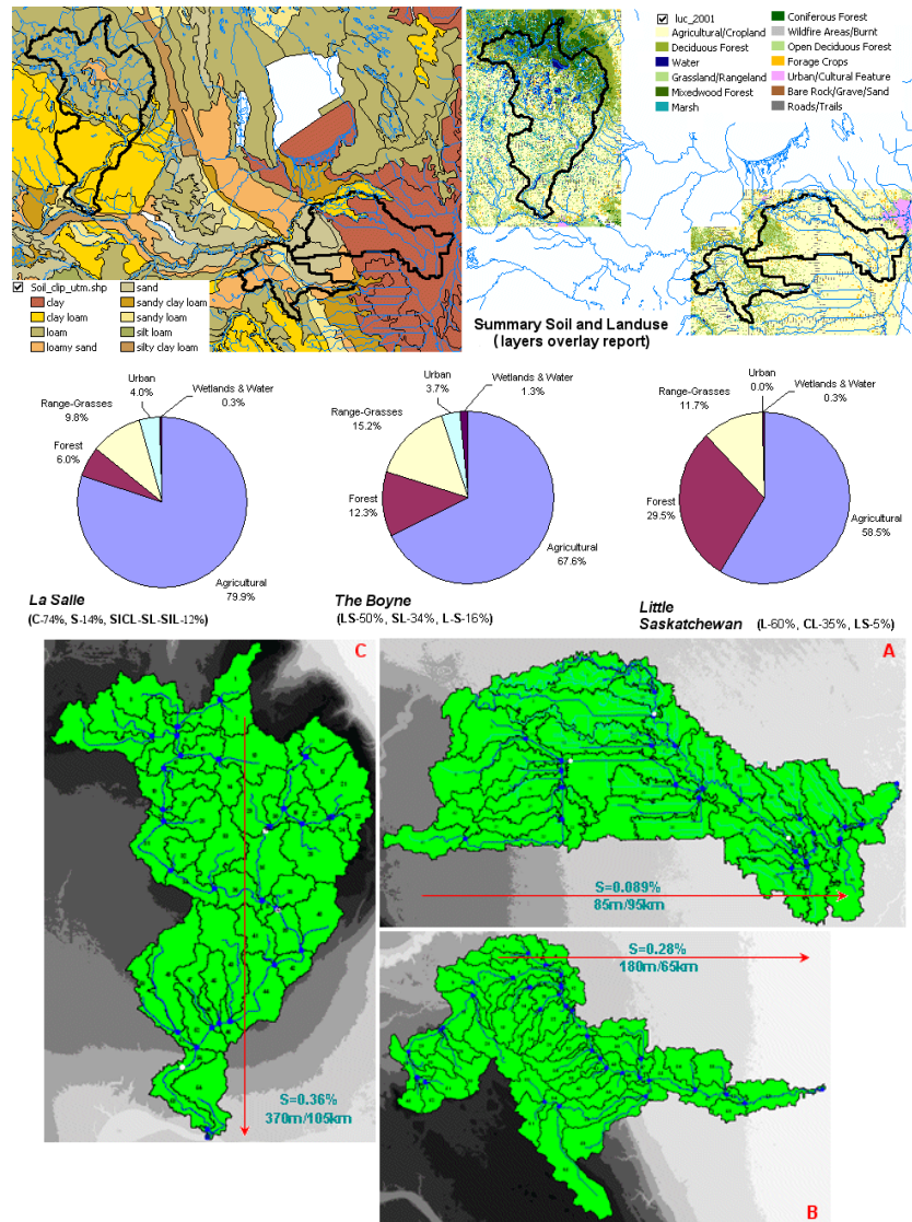
Figure 2. Digital maps and SWAT watershed delineation for pilot watersheds - top: soil and land maps; middle: land use plots and soil type percentages; bottom: DEM-delineation on targeted watersheds: A) La Salle, B) Boyne, and C) Little Saskatchewan.
