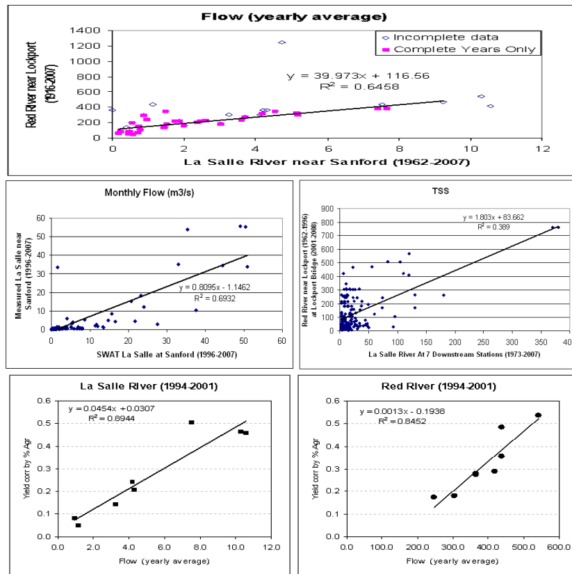
Figure 6. La Salle and Red rivers regressions: top) yearly average flow; mid) monthly flows and TSS; bot) yearly average TP yield (kg/ha AGR/yr)
