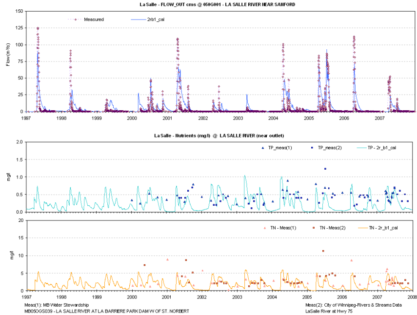
Figure 4. Daily SWAT output against measured values for flow and nutrients in the La Salle River basin (top: daily flows near Sanford; bottom: nutrients at the watershed outlet)
