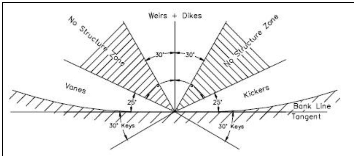
Figure 2-3. Bendway Weir and Vane Variations.
