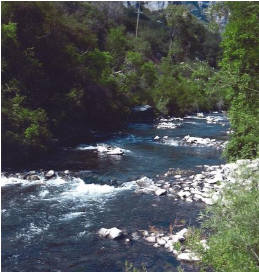
Figure 2-4. Bendway Weirs on the Provo River.
