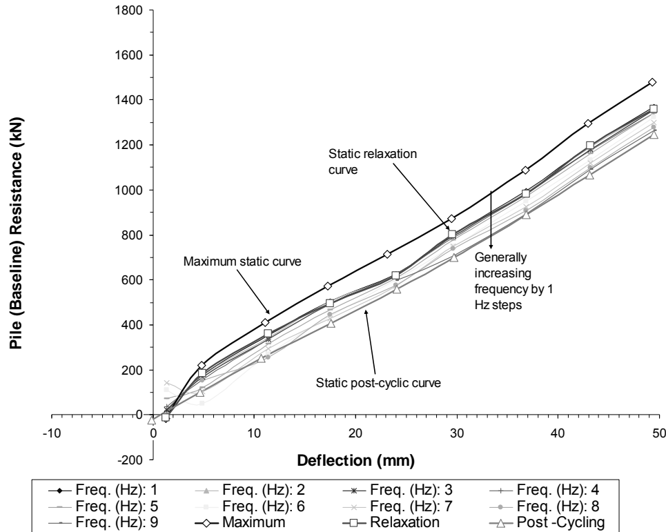
Figure 4-11 Relaxation Effects and Dynamic, Cyclic Effects on Total Passive Resistance as a Function of Frequency
