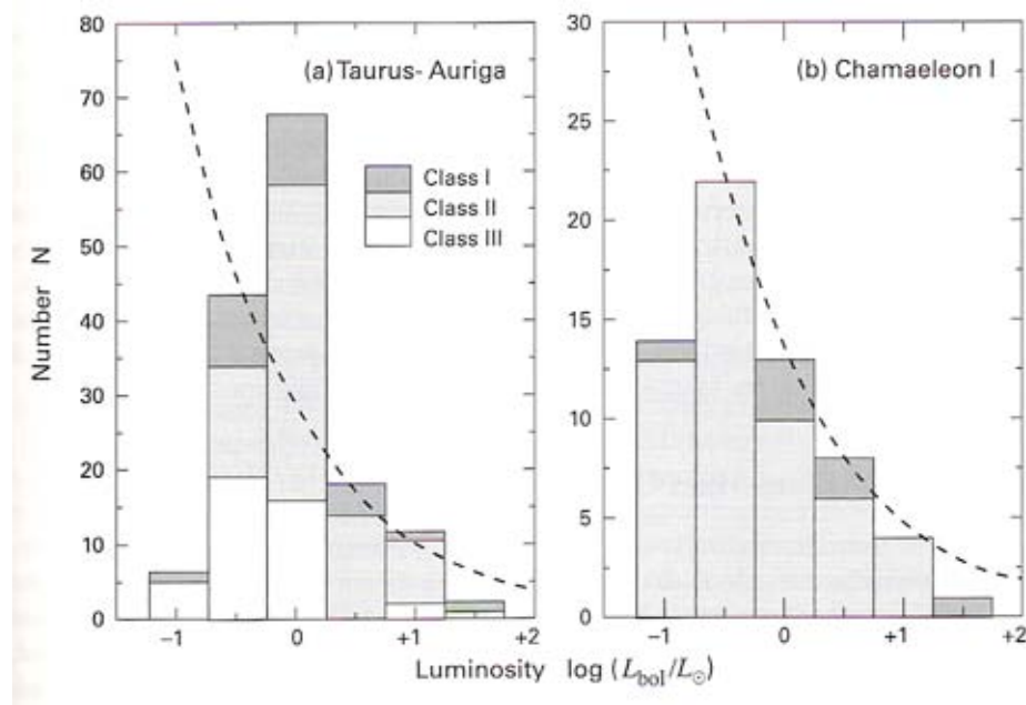
Figure 67: Bolometric luminosity functions for (a) Taurus-Auriga and (b) Chameleon I. The dashed curve is the initial luminosity function, defined here as the relative number of field stars per logarithmic unit of L_{\text{bol}} . Shading indicates different infrared classes, as explained in panel (a). Figure 4.13 in Stahler and Palla
