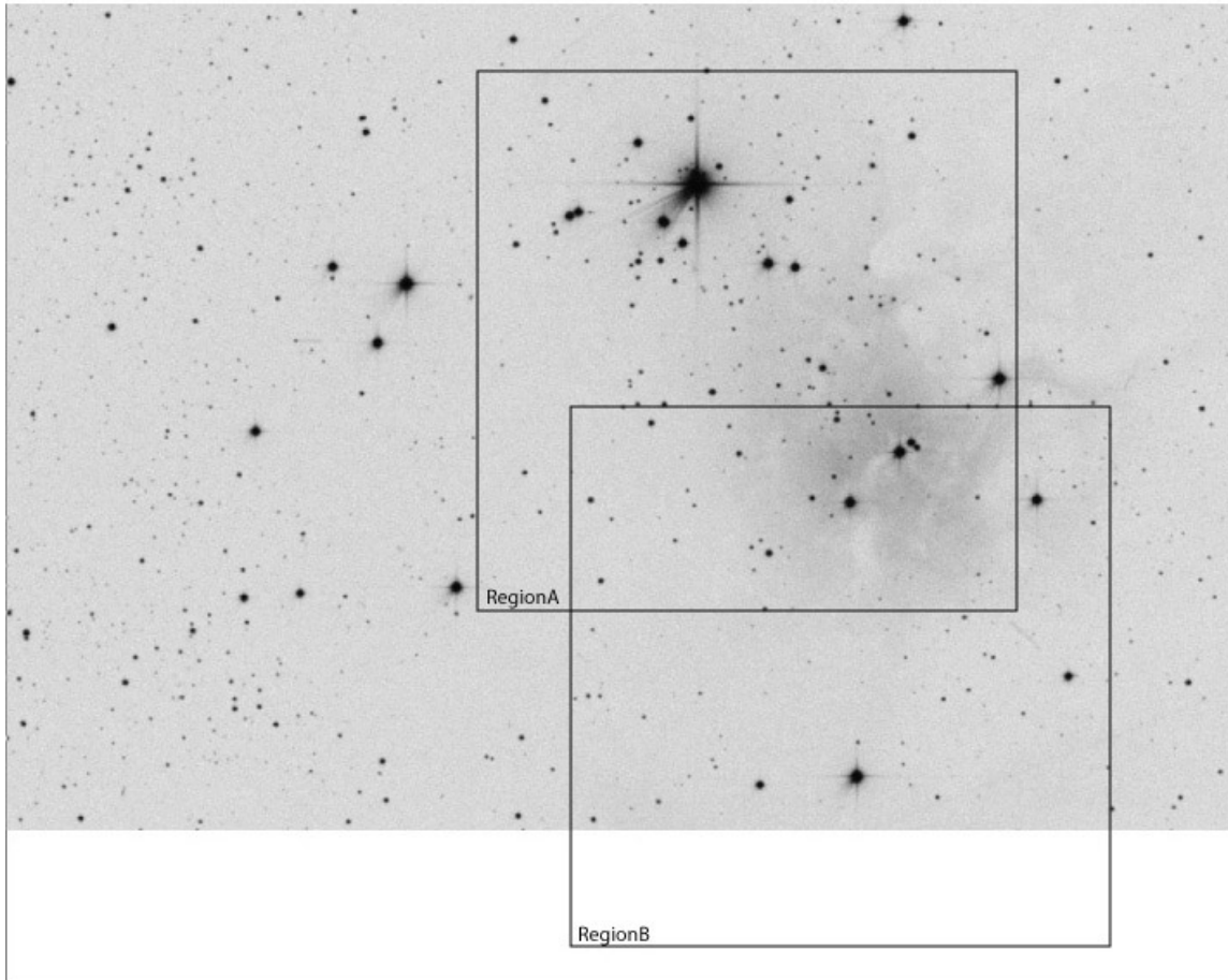
Figure 7: The NGC 2264 as observed from Tenagra Observatory. Two separate regions, as indicated, were observed. For the stars in the overlapping region, the observations were averaged.
