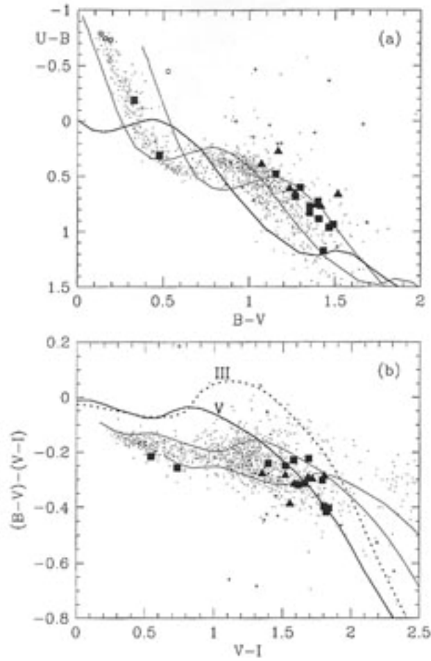
Figure 3: Figure 4 in Sung 1998. Color-color diagrams. The thick lines represent the ZAMS relation, while the two thin solid lines represent reddened ZAMS relations for E(B - V) = 0.35 and 0.7 mag, respectively. The other symbols are the same as in Figure 6. These color-color diagrams were used to attempt to determine the locus of the MS. As the locus of the MS is not clearly visible these combinations were abandoned for those of Figure 8.
