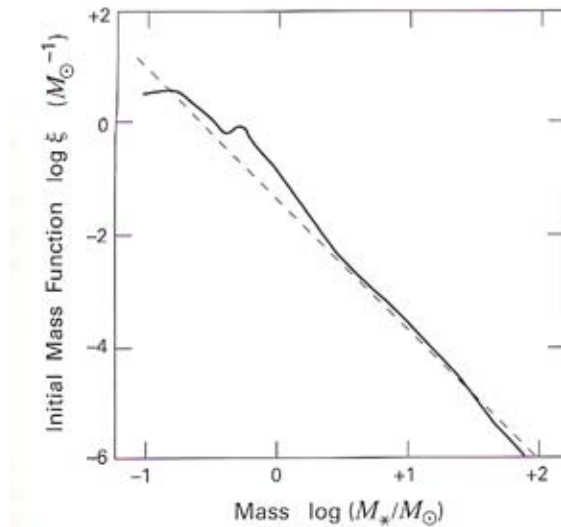
Figure 66: Initial mass function for solar neighborhood stars. The dashed line has the same slope as Salpeter's power law. Figure 4.22 in Stahler and Palla
