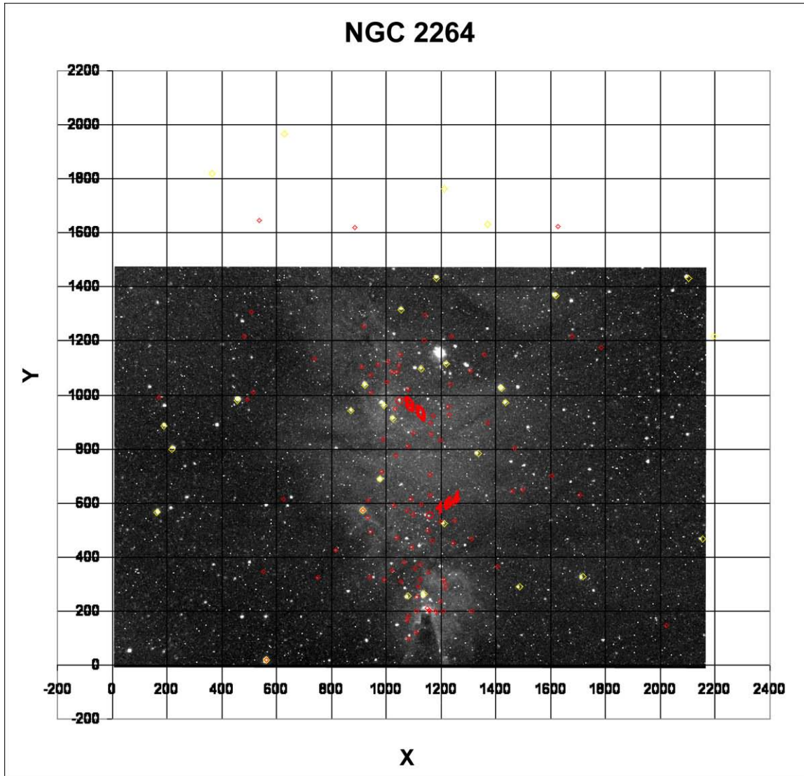
Figure 33: Coordinates of objects for NGC 2264. Coordinates have been overlaid with a representative H \alpha image of the cluster. Yellow stars are the 30 brightest main-sequence objects and red squares indicate emission candidates. The two numbered stars are those for which spectra were obtained at DAO.
