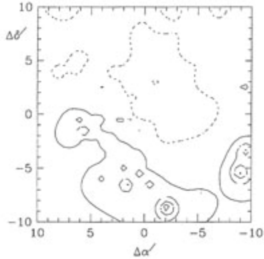
Figure 1: Figure 5 in Sung 1998. Reddening distribution of NGC6231. The dotted (upper section), solid, dashed, dot-dashed, and long-dashed lines represent E(B-V) = 0.45, 0.50, 0.55, 0.60, and 0.65 mag, respectively. In practice a map such as this is very difficult and time consuming to create. Once made however, the location of a star in a certain region allows for the proper reddening correction ( E[B-V] ) to be determined and used in calculating the color for that star.
