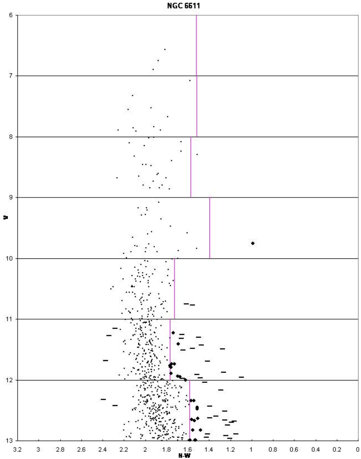
Figure 47: V vs. N-W for NGC 6611. Outliers are shown with dashes. Those outliers are to the right of the main-sequence are emission candidates. Additional emission candidates are given as dots. These are objects located to the right of the pink selection lines. The selection lines are drawn at 2\sigma from the mean of the main-sequence for that V magnitude range.
