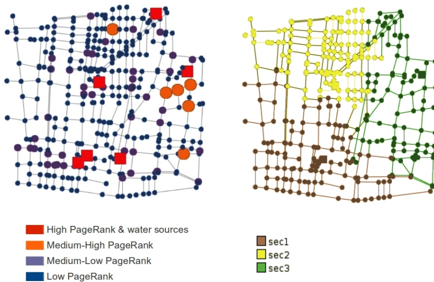
Figure 2: Spectral sectorisation and PageRank distribution in the case-study.
