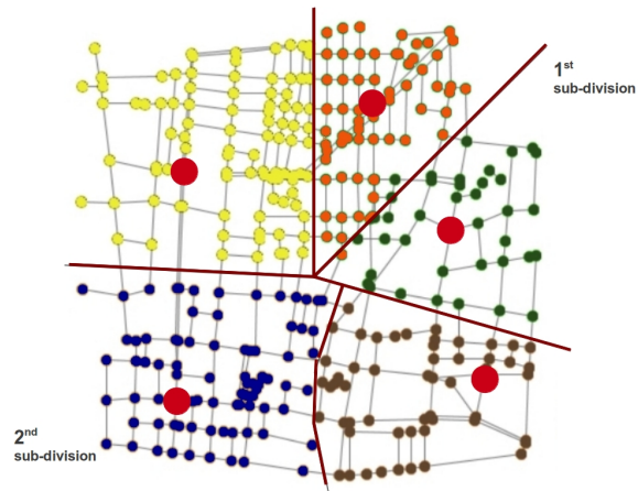
Figure 3: Final location of 5 sensors in the WSN of our case-study.
