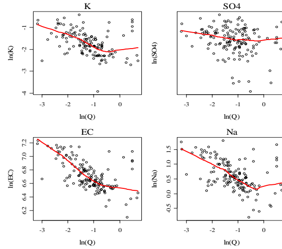
Figure 2: Scatter plots of Ln-transformed water quality variables against Ln-transformed flows for the Ziarat River
